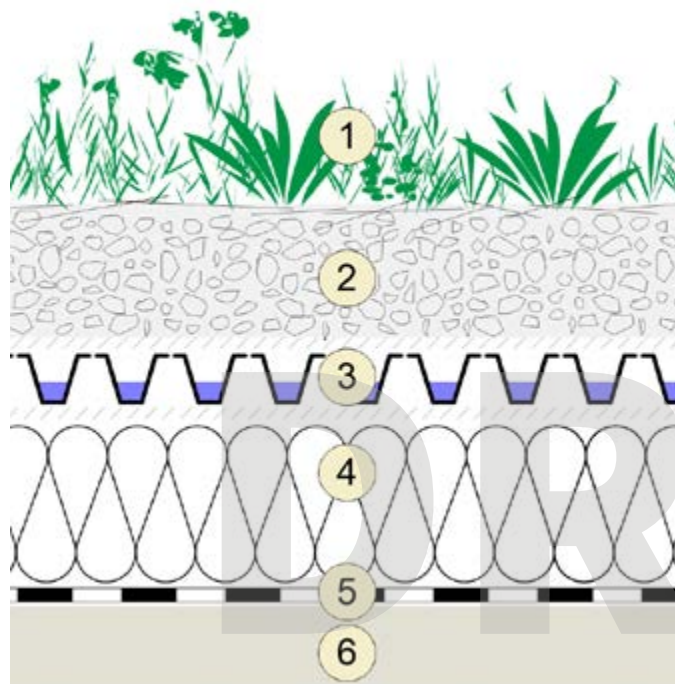
Figure 8: Construction layers of a green roof (Source: Auraplan)
